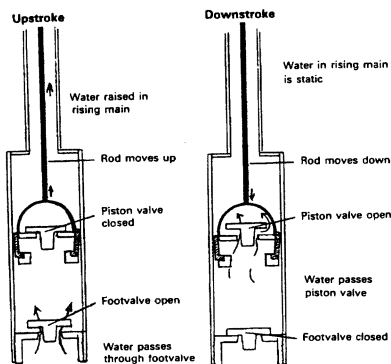
FIGURE 2 Hydraulics
